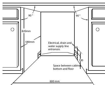
Cabinet Dimension
