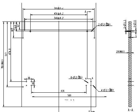
Shutter Dimension
